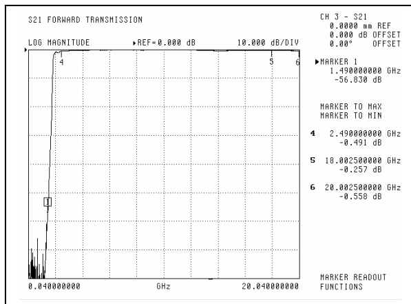
Amplitude Response
